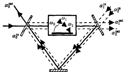
图 1 NOPO 示意图( \alpha_0^i, \alpha_1^i, \alpha_2^i 分别为输入的抽运场,信号场和闲置场; \alpha_0^o, \alpha_1^o, \alpha_2^o 为输出场)
